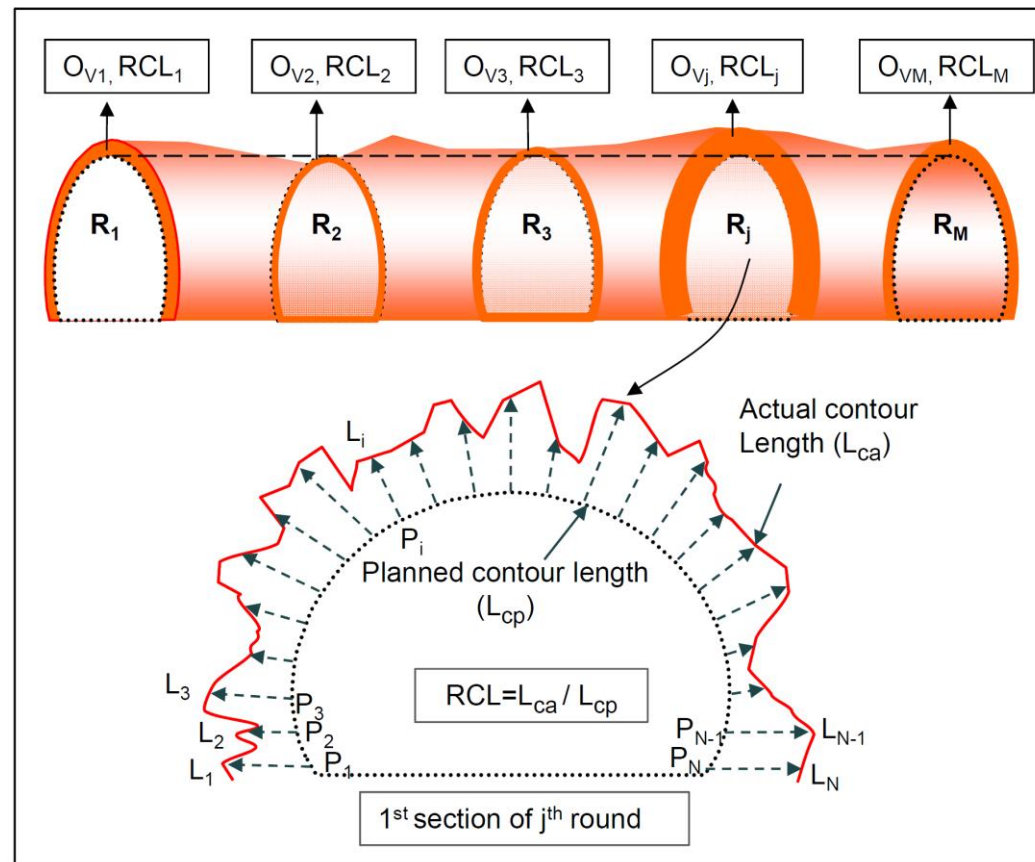
Figure 3.3. Definition of variables for TCI
